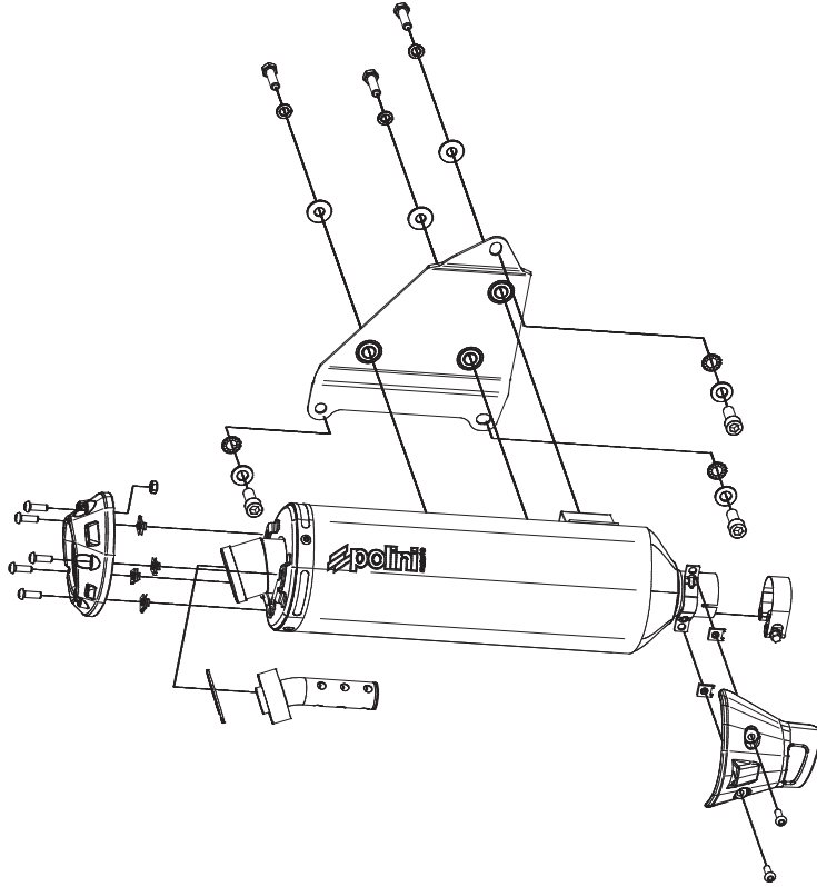
Silencer
